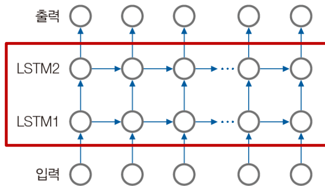
(a) 적층 LSTM
