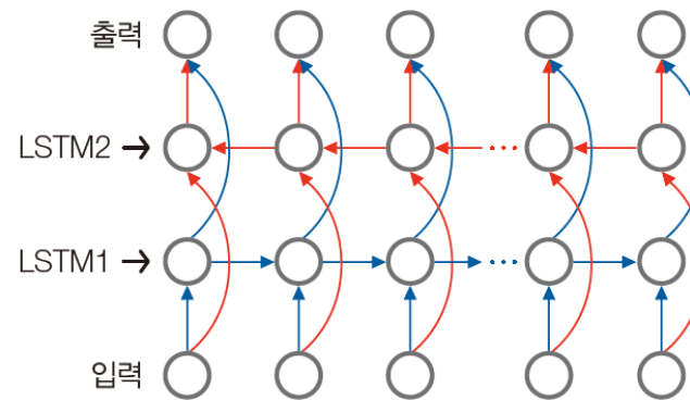
(b) 양방향 LSTM
